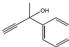
1-PHENYL-1-PROPYN-1-OL
