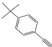
4-(T-BUTYL)PHENYLACETYLENE-
