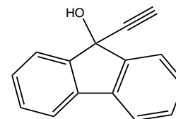
9-ETHYNYL-9-FLUORENOL
