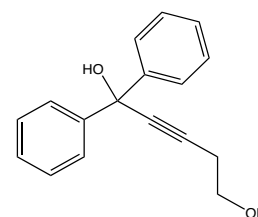
1,1-DIPHENYL-2-PENTYN-1,4-DIOL
