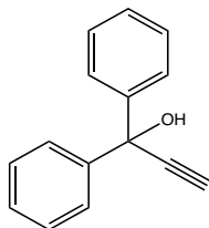
1,1-DIPHENYL-2-PROPYN-1-OL
